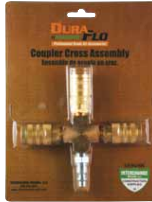
Coupler Cross Assembly 1/4" Industrial 90510 CX-I 1/4" Automotive 90505 CX-A 3/8" Industrial 90515 CX38-I 3/8" Automotive 90516 CX38-A
