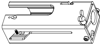
98744/WKT013: Body and End Plate
