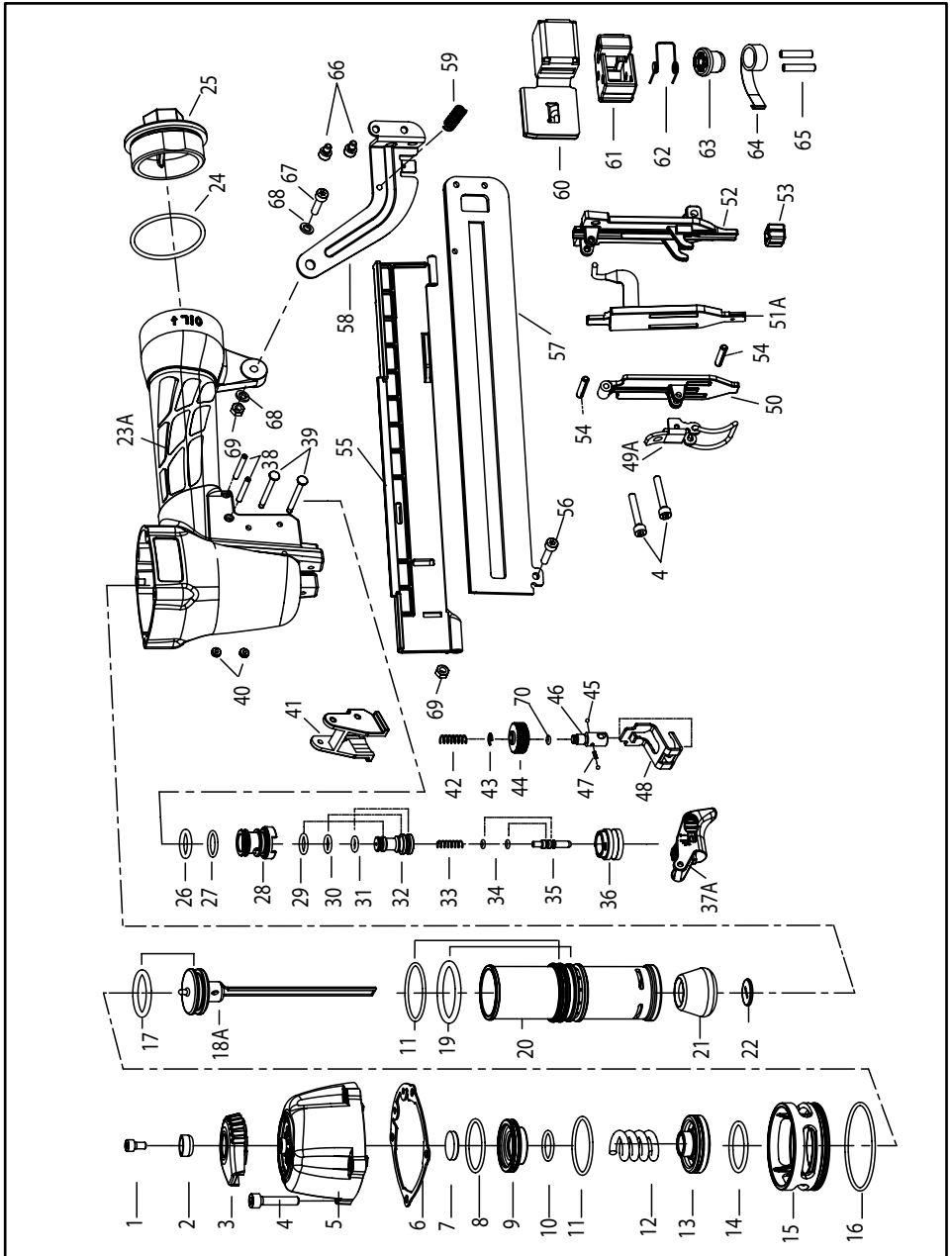
SL4018 Parts Drawing (01-01-13)
